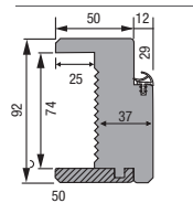
KM1 cloison 72 mm recouvrement
